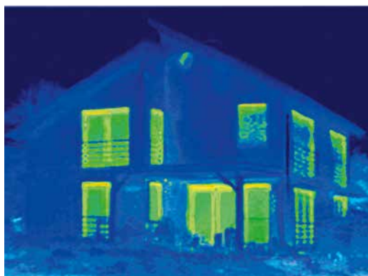
Thermal imaging shows the major energy benefits of investing in carefully installed new windows from the Schüco LivIng window system. Almost all of the original energy losses are completely avoided.
